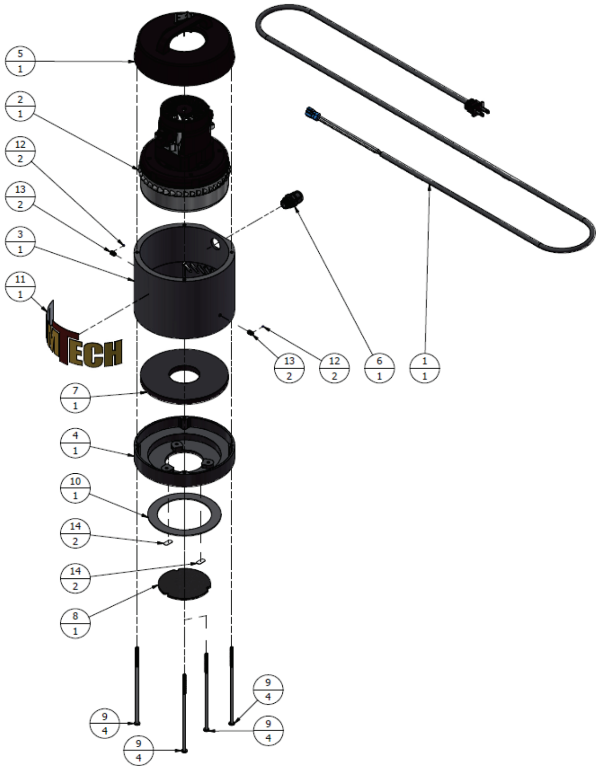
2.13 VP-225HV/A – ASSY, VACUUM MOTOR, 110V, HI-VAC (Parts ID)
