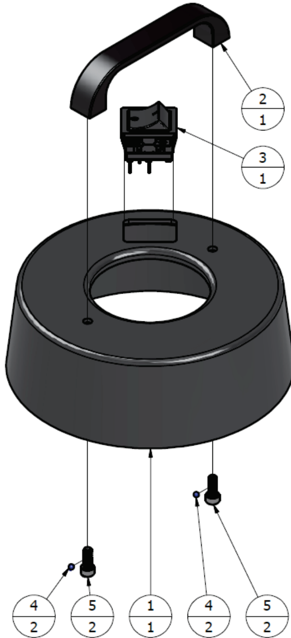
2.19 VP-240HV.2/A – ASSY, LID, VACUUM MOTOR, 220V, HI-VAC (Parts ID)
