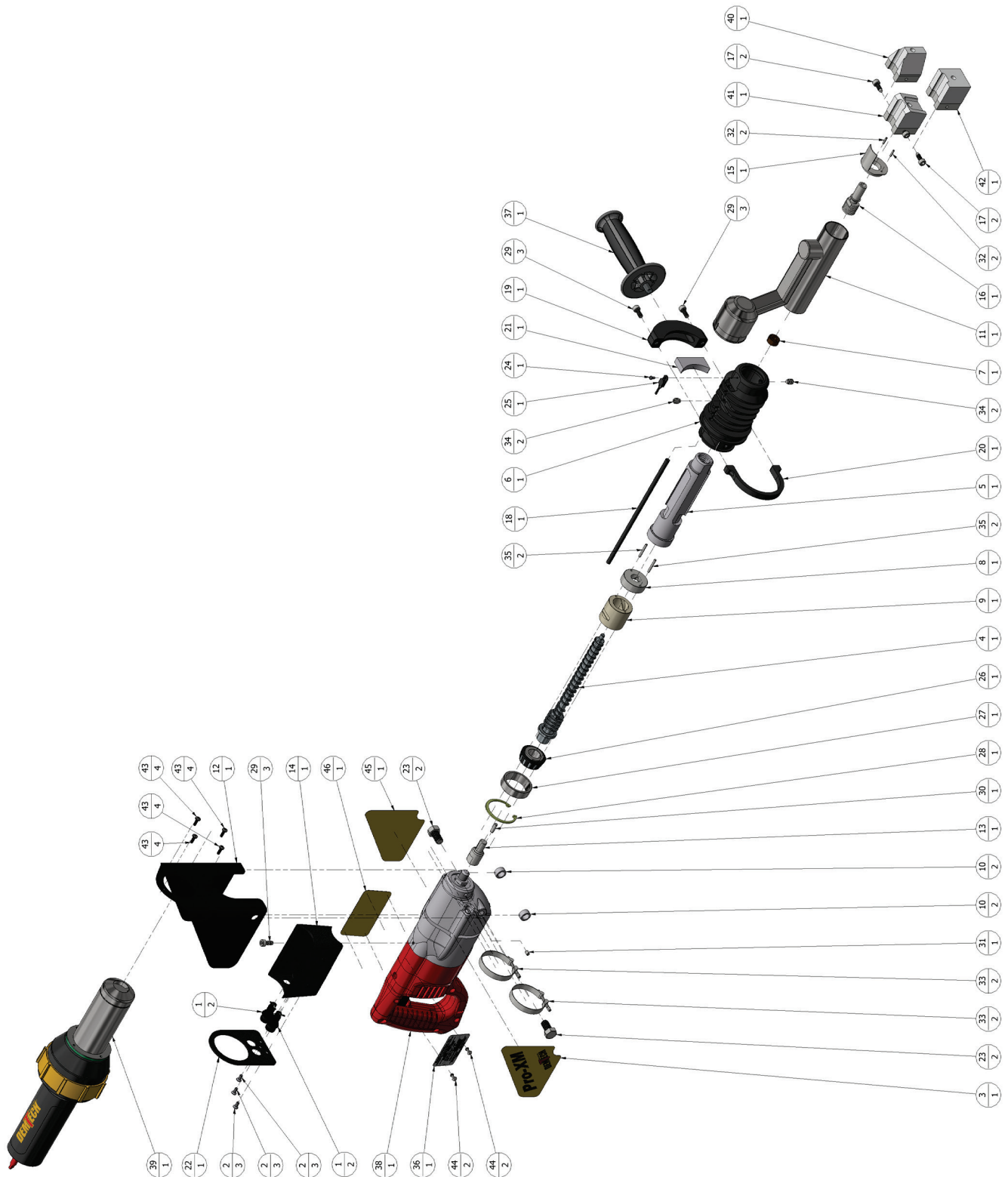
1.1 605-0100/PRT/A – ASSY, PRO-XM EXTRUSION WELDER (Parts ID)
