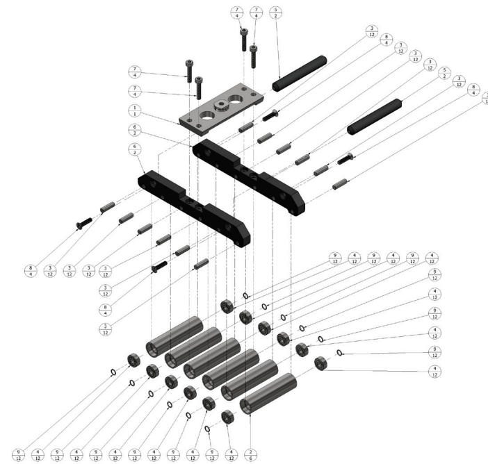
1.18 500-120.6/3XL/A - ASSY, CONTOUR ROLLER, LOWER (Parts ID)
