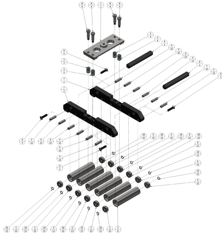
1.18 500-120.6/3XL/A - ASSY, CONTOUR ROLLER, LOWER (Parts ID)
